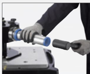
Mounting sleeve
