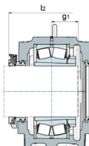
Taconite seal TA Cover TE
