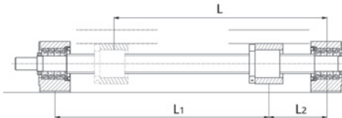
Figure 2.17 __ Bearing arrangement fixed - fixed
