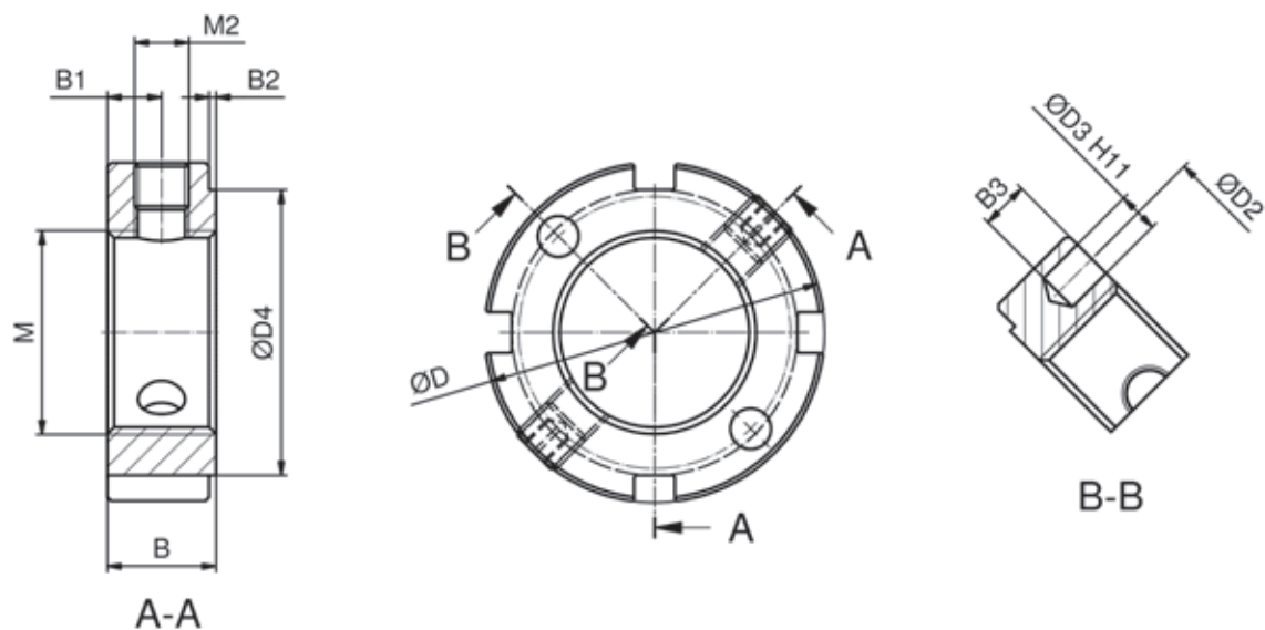
Figure 6.8 ____ Dimension self-locking precision PRS
