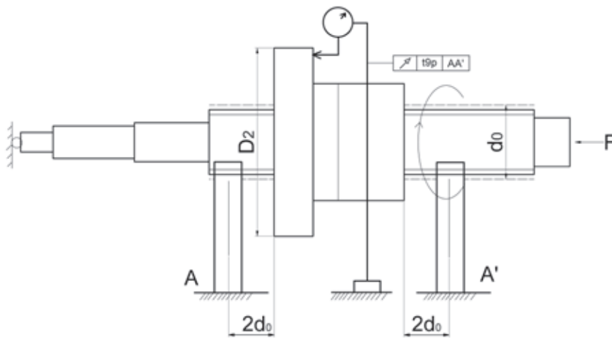
Figure 2.9 __ Measurement of the axial runout t_g of the contact surfaces of the Ball Screw nut
