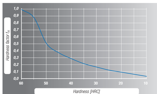
Figure 2.19 _ Hardness factor f_H
