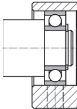
Figure 6.13 __ Dimension floating bearing unit BF and EF
