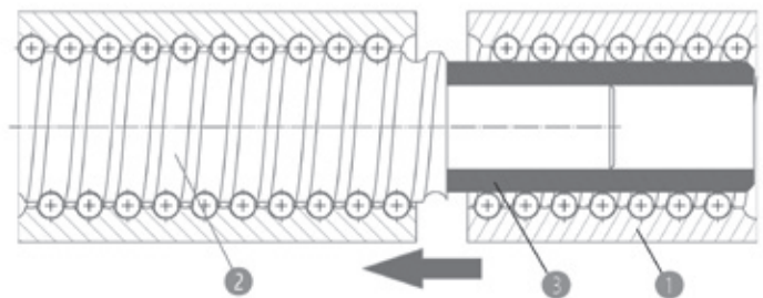
Figure 3. ____ Assembly of Ball Screw nuts
