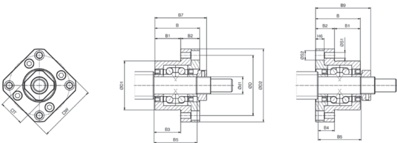
Figure 6.12 __ Dimension fixed bearing units FK
