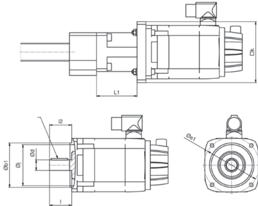
Figure 6.23__ Dimension of standard coupling cones for BSTK bearing units
