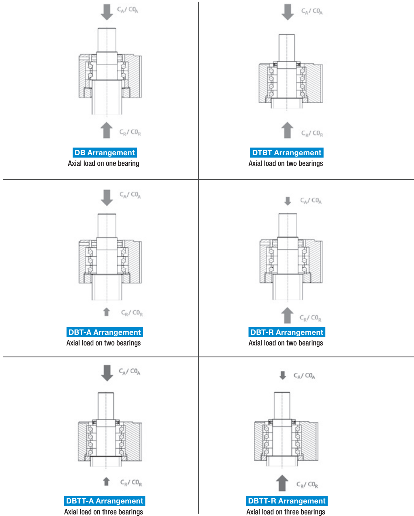
Figure 6.3 Bearing arrangement in fixed bearing units BSTK
