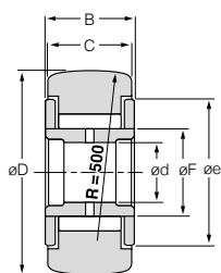
NATV (sans cage)
