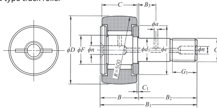
KRV type (Full complement roller type)
