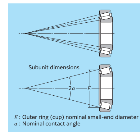
Fig. 1.5 Tapered roller bearings
