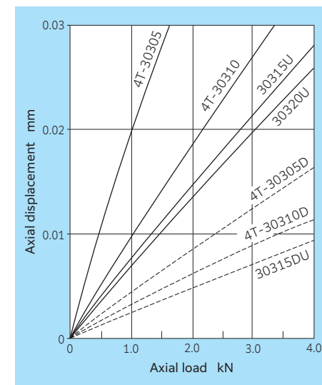
Fig. 17.2.9 Series 303/303 D axial load vs. axial displacement
