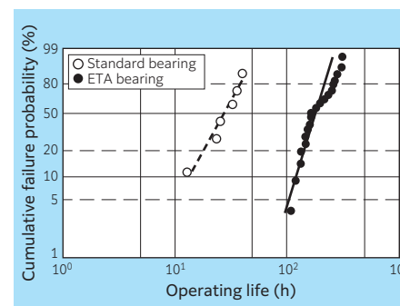
Fig. 13.4 Operating life comparison between ETA tapered roller bearing and standard bearing (mixed with foreign matter)
