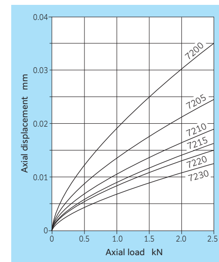
Fig. 17.2.3 Series 72 axial load vs. axial displacement
