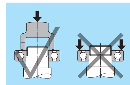
Fig. 15.11 Press-fitting bearing into shaft
