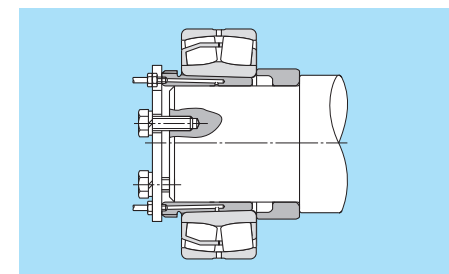
Fig. 15.23 Installation using hydraulic withdrawal sleeve
