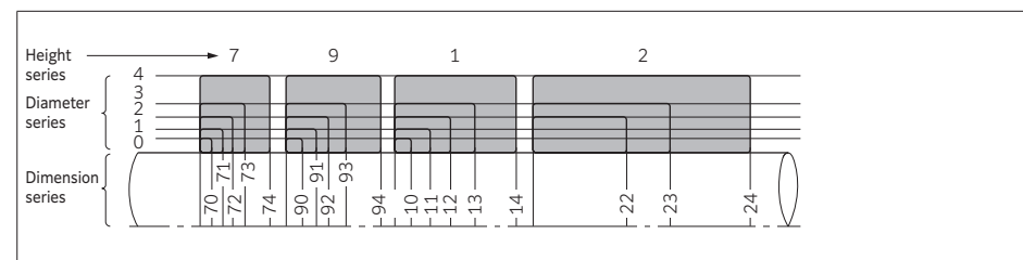
Fig. 5.6 Dimension series for thrust bearings (excluding diameter series 5)
