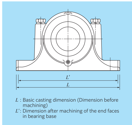
Fig. 1 Seating surface length dimension of plummer block
