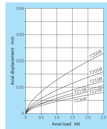
Fig. 17.2.4 Series 72 B axial load vs. axial displacement
