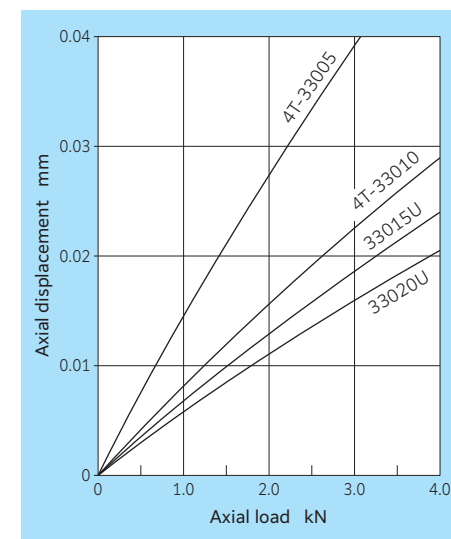
Fig. 17.2.10 Series 330 axial load vs. axial displacement
