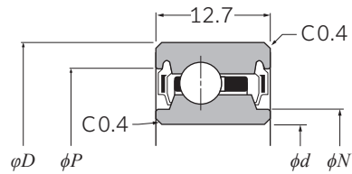
Radial type (with double-seal)
