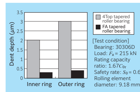
Fig. 13.14 Measurement result of dent depth
