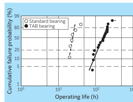
Fig. 13.3 Operating life comparison between TAB deep groove bearing and standard bearing (mixed with foreign matter)
