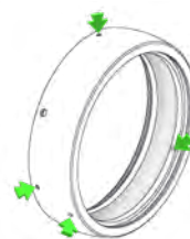
Figure 1 G2 system: Outer ring with four lubrication holes in two planes
